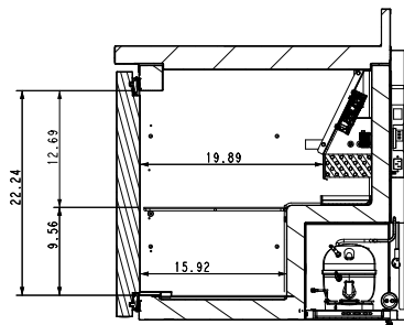
SIDE VIEW ALL MODELS
