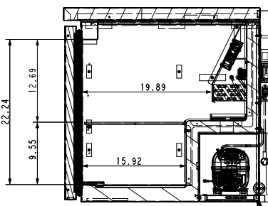
SIDE VIEW ALL MODELS
