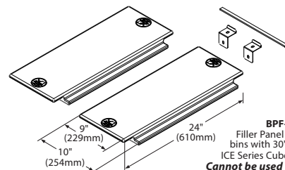
KBT222 Bin Top for 48" (1219mm) bins with (2) 21" (533mm) wide GEM Series Ice Makers & MFI Series Ice Makers
