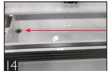
14 Drain hole.
