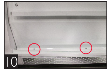
10 Example of screws to remove.
